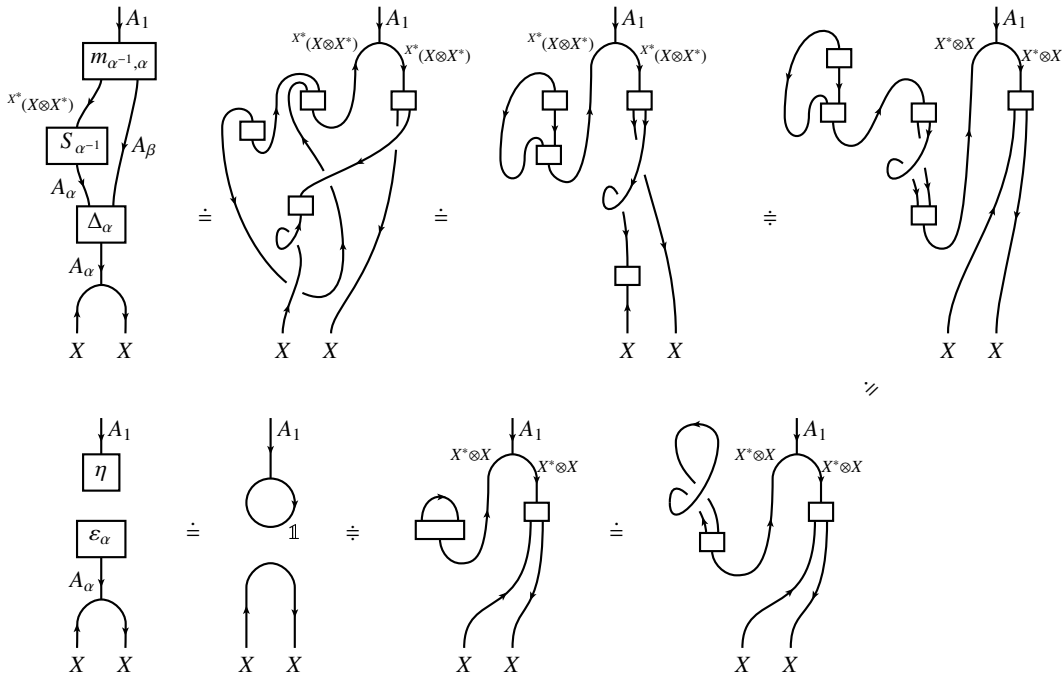
FIGURE 3.18. m_{\alpha^{-1},\alpha}(S_{\alpha^{-1}} \otimes \text{id}_{A_\alpha}) \Delta_\alpha i_X = \eta \varepsilon_\alpha i_X
