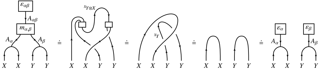
FIGURE 3.17. \varepsilon_{\alpha\beta} m_{\alpha,\beta}(i_X \otimes i_Y) = (\varepsilon_\alpha \otimes \varepsilon_\beta)(i_X \otimes i_Y)
